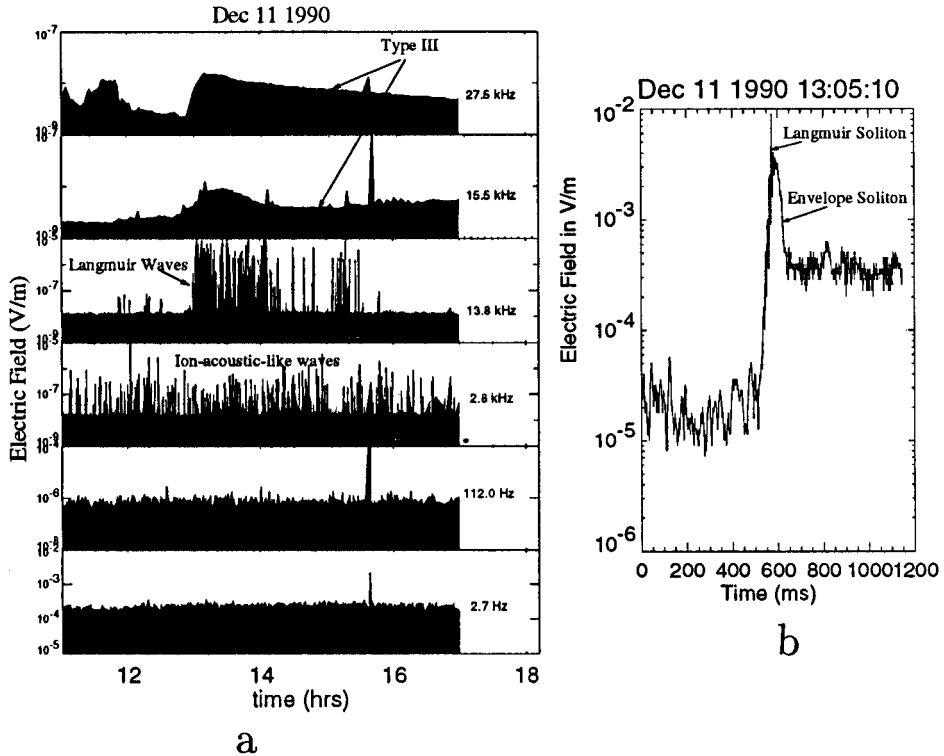
Fig. 1. Radio and in situ plasma wave phenomena
