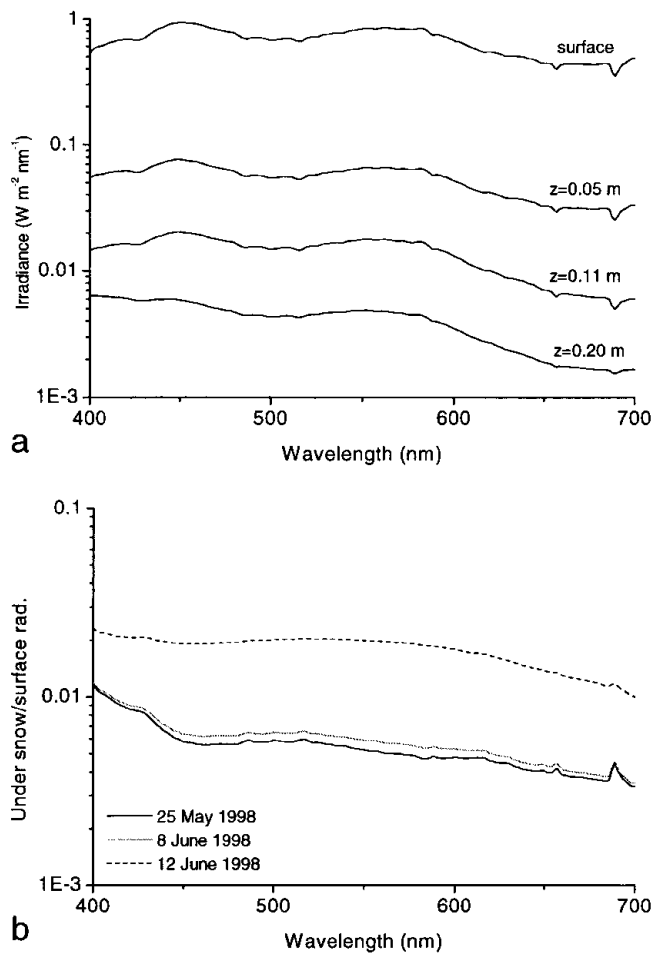
Fig. 4. Measurements of spectral incoming radiation under snow in the PAR wavelength range, measured at site B. For all measurements the sky was 8/8 cloud-covered (overcast conditions). (a) Spectra at the surface, and at three different depth levels under snow (0.05, 0.11 and 0.20 m), measured on 8 June 1998. The curves show that the spectral composition is little changed within the PAR range under these conditions. (b) Spectra of attenuated radiation under snow in the PAR wavelength range, measured on 25 May, 8 June and 12 June 1998. The measurement depth on the first two dates was 0.20 m, and on 12 June it was 0.19 m. This last curve was corrected so as to be comparable with the first two curves. The 12 June measurement shows more attenuation at wavelengths of < 500 nm, compared with the spectra measured earlier. This may be due to impurities in the surface snow layer. The glitch at 690 nm is probably a spectrometer-specific error.
