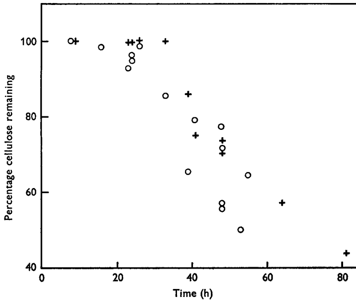
Fig. 2. Breakdown of cellulose in the rumen (+) and the caecum (O) of sheep.
