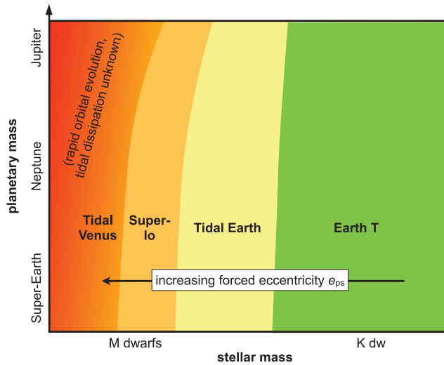
Figure 3. Schematic classification of hypothetical 10 M_{\text{Gan}} -mass ( \approx 0.25 M_{\oplus} ) moons in the widest Hill stable orbits about planets in the stellar IHZ. In the IHZ about M dwarfs a satellite’s eccentricity e_{ps} is strongly forced by the close star, which induces strong tidal heating in the moon. A Tidal Venus moon is uninhabitable.
