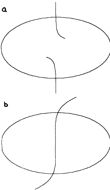
Figure 1: Appearance of a dust lane (open curve) relative to the stellar figure (ellipse) formed by a) capture in the unstable polar orbit of an oblate figure, b) capture in the stable periodic orbit of a triaxial figure.
