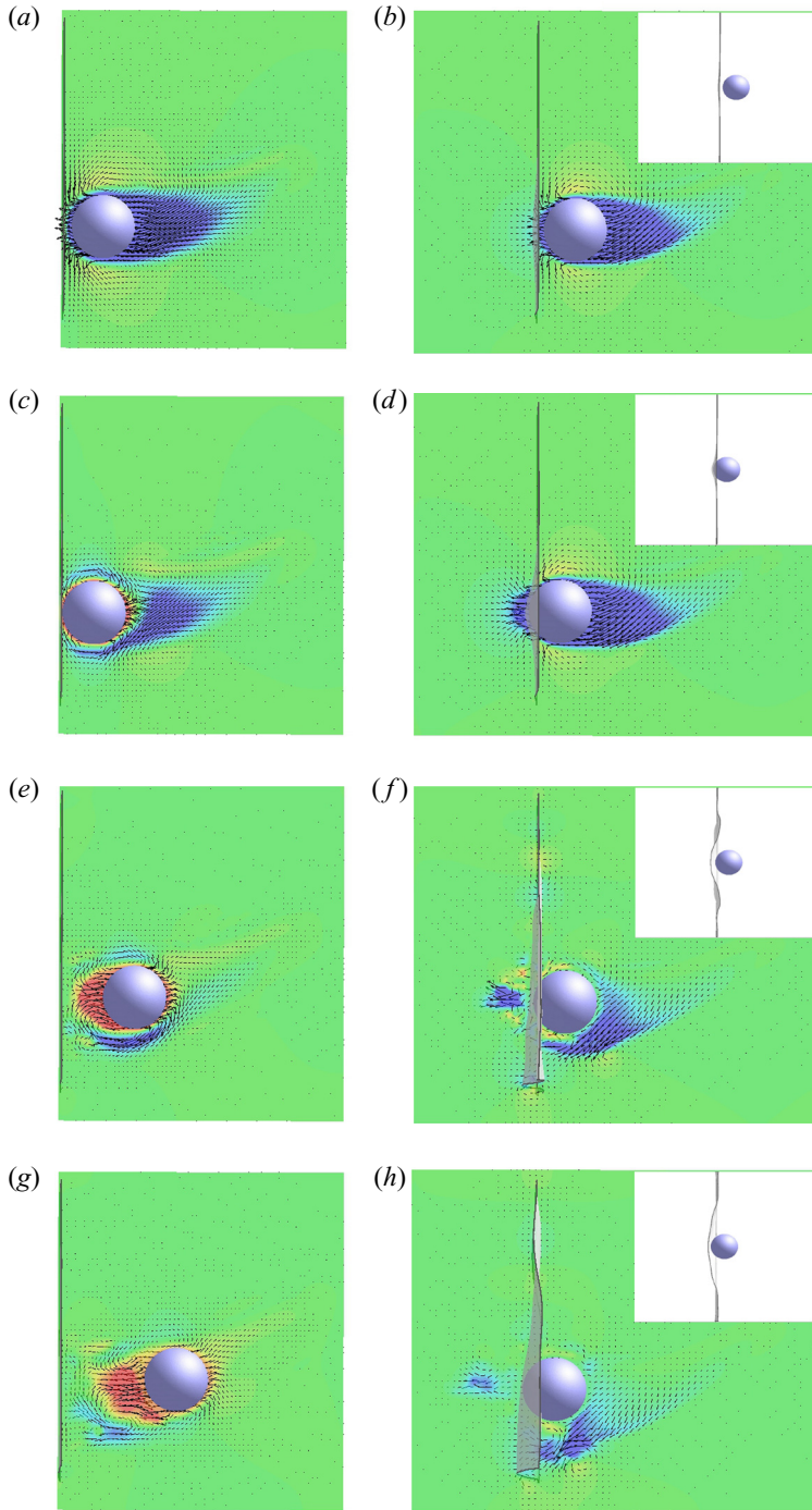
Figure 10. Comparison of the numerical results for the pendulum interaction with a solid block e/(2R) = 10 (a,c,e,g) and a membrane e/(2R) = 0.1 (b,d,f,h) for a case at Re = 1000 and \rho_p/\rho_f = 8 ; (a,b) t = 4.0 , (c,d) t = 4.2 , (e,f) t = 5.0 , (g,h) t = 6.0 . Snapshots in the y - z -plane; the contours represent the u_z velocity component with the colours blue to red for -1 \leq u_z \leq 1 . Also the velocity vectors are overlaid and only one in every three grid points are reported for clarity. The insets of the panels (b,d,f,h) show the structures from below.
