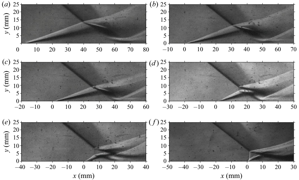
Figure 15. LESF fields at Mach 5.52 with 26.6° wedge. The shock impingement location is varied in the range 10–60 mm from the plate leading edge: (a) X_{ir} \approx 60 mm; (b) X_{ir} \approx 50 mm; (c) X_{ir} \approx 40 mm; (d) X_{ir} \approx 30 mm; (e) X_{ir} \approx 20 mm; (f) X_{ir} \approx 10 mm.
