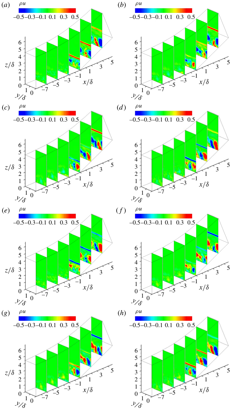
FIGURE 11. Pure oscillation based on mode LF3. One period of the dynamics is shown using eight uniformly spaced snapshots.
