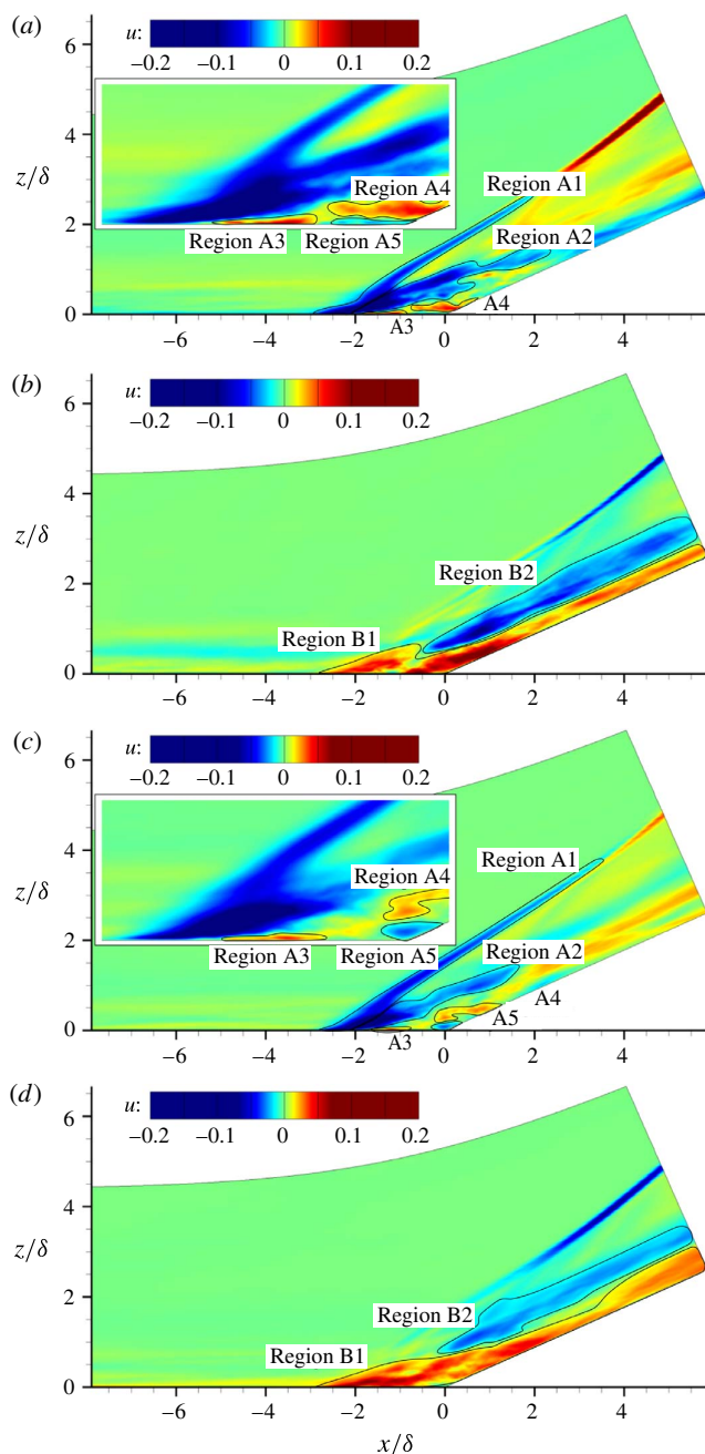
FIGURE 16. Two-dimensional field of u perturbation obtained by spanwise averaging the reconstruction of the dynamics based on the 3-D DMD modes LF1–LF5. Snapshot (b) occurs \Delta t U_\infty / L_{sep} = 5.6 after snapshot (a) and snapshot (d) occurs \Delta t U_\infty / L_{sep} = 3.2 after snapshot (c). The first pair of snapshots (a,b) is uncorrelated with the second pair (c,d).
