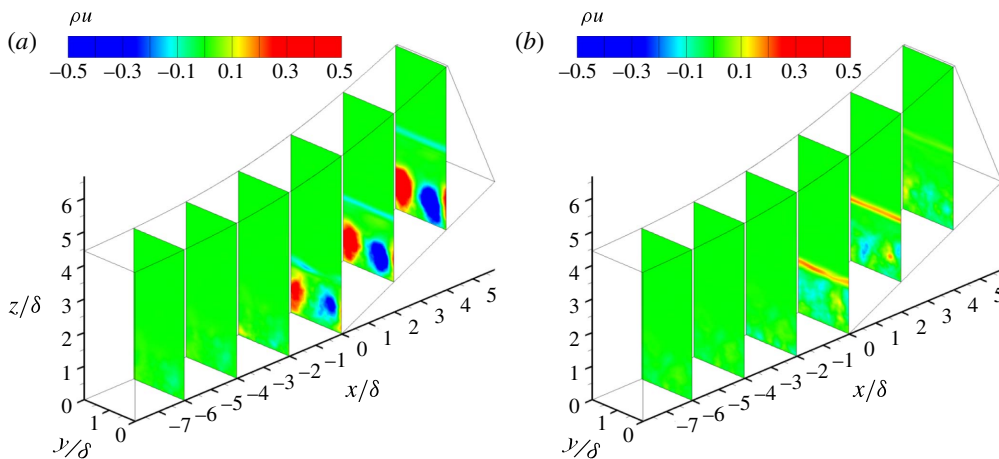
FIGURE 8. Low-frequency DMD mode LF1 visualized by contours of the streamwise mass flux \rho u . (a) Real part and (b) imaginary part.
