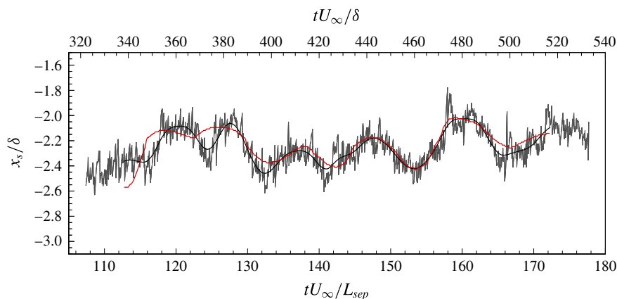
FIGURE 13. Comparison between the original DNS data and the reconstruction based on all of the relevant low-frequency DMD modes. The comparison is shown in terms of the separation point x_s . The DNS is shown in black, and the reconstruction based on modes LF1, LF2, LF3, LF4 and LF5 in red. Note that this figure is identical to figure 1, except that the DMD reconstruction has been added.
