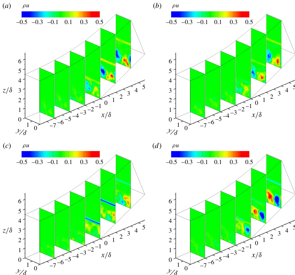
FIGURE 14. Reconstruction of the low-frequency dynamics based on modes LF1, LF2, LF3, LF4 and LF5. Four uncorrelated snapshots are shown. In addition, a movie of the reconstruction is available with the online version of this paper.
