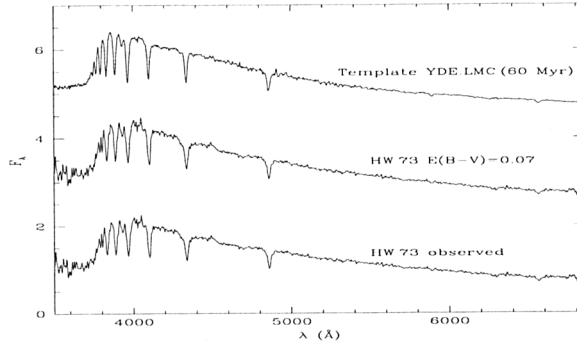
Figure 1. Observed integrated spectrum of HW 73, the reddening-corrected spectrum ( E(B-V)=0.07 ), and the template which best matches it. Spectra are in relative flux units normalized at \lambda=5800\text{\AA} .
