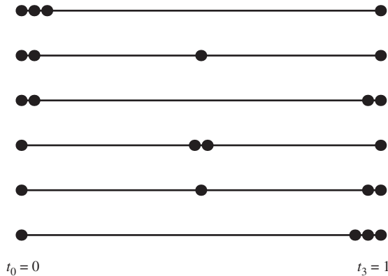
FIGURE 1. All possible cases for n = 3 .
