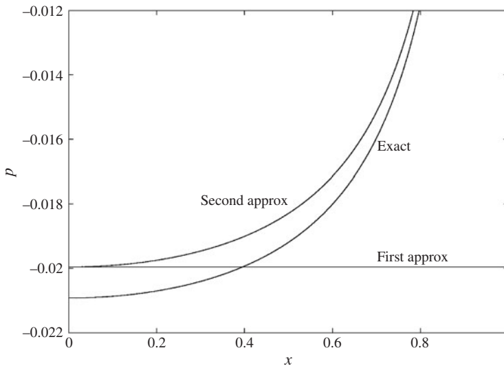
FIGURE 5. Pressure p(x) on spheroid with slenderness \epsilon = 0.1 .
