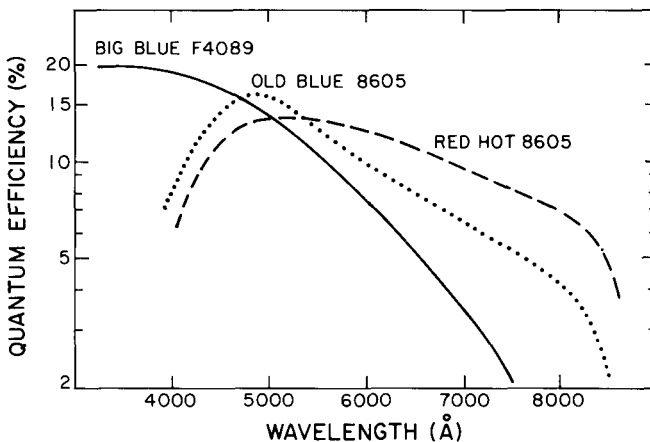
Figure 2. Measured cathode sensitivities
