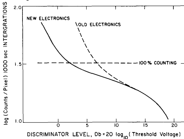
Figure 3. Integrated pulse-height distributions
