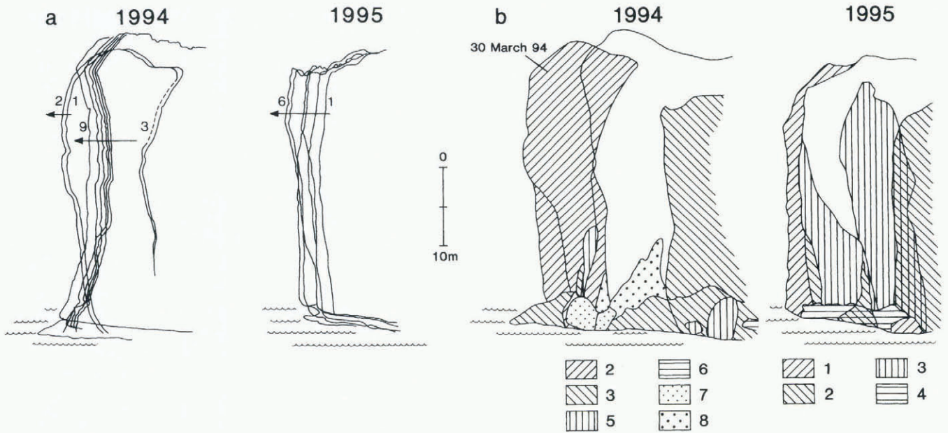
Fig. 3. (a) Short-term changes in ice-cliff position traced from superimposed colour slides. Numbers refer to order of photographs: 1994: 1=29 March; 2=30 March; 3=31 March; 4=7 April; 5=8 April; 6=9 April; 7=10 April; 8=12 April; 9=12 April. 1995: 1=18 March; 2=21 March; 3=24 March; 4=24 March; 5=26 March; 6=27 March. (b) Distribution of ice calved from the cliff. Numbers refer to periods between photographs. The calving event of 31 March 1994 is indicated (see text).
