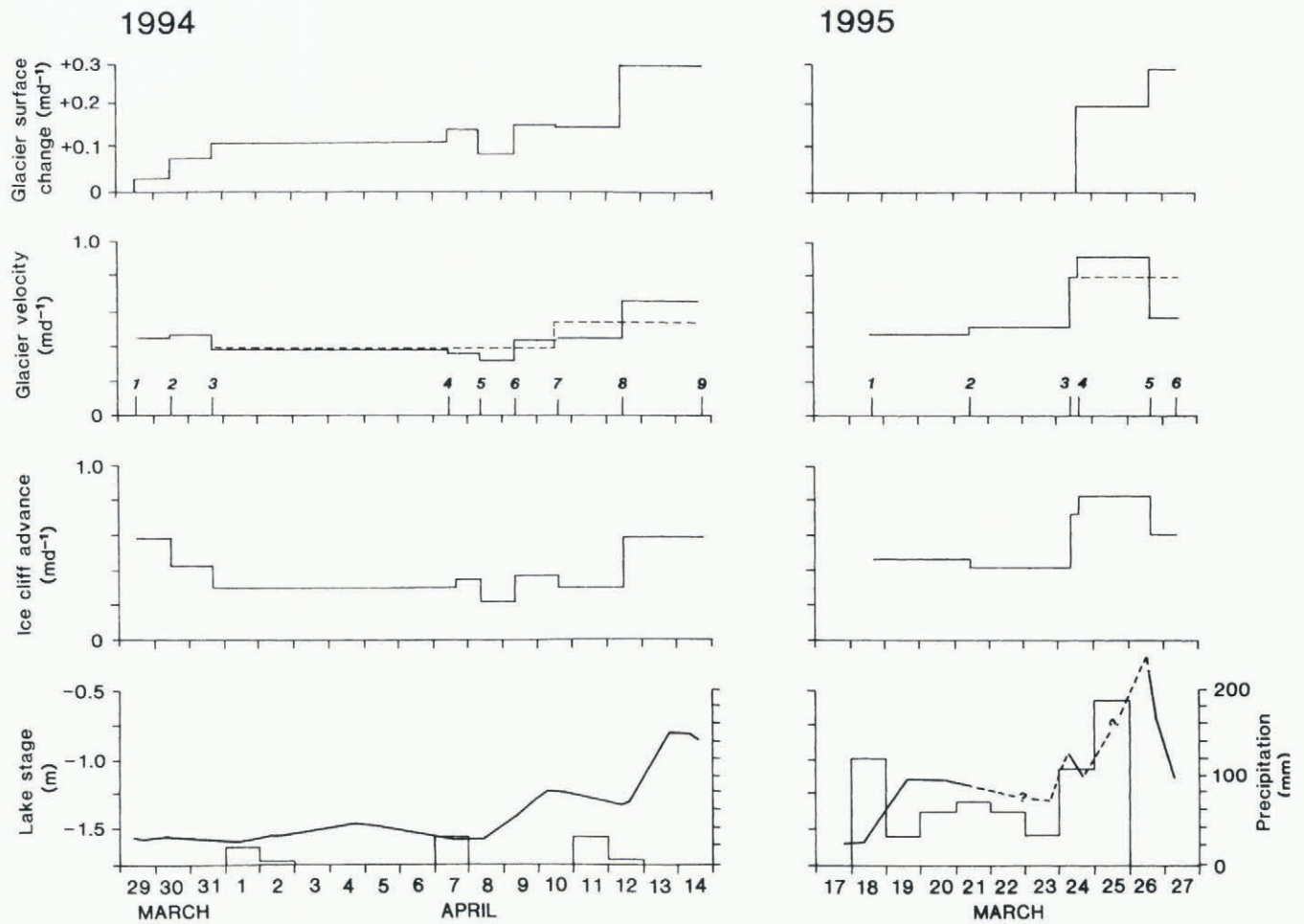
Fig. 4. Time series of glacier surface change, velocity, ice-cliff advance and lake stage for Maud Glacier in the 1994 and 1995 austral autumns. Numbers in italics refer to photographs (see Fig. 3a caption). Dashed lines show surface velocity measured by theodolite survey. Precipitation data are from Mount Cook village.
