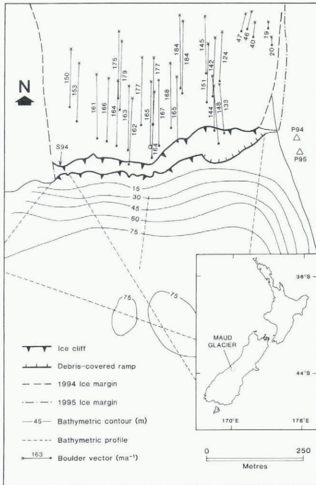
Fig. 1. Map of the terminus region of Maud Glacier showing locations of photo stations, ice cliff in 1994 and 1995, markers used for velocity surveys, and ice-proximal bathymetry based on echo-sounding survey. Boulder vector shown by open circle was surveyed in the field; the rest were measured by aerial photogrammetry. Site of ablation stake in 1994 marked "S94". Map drawn from corrected near-vertical aerial photographs taken on 16 April 1994 and 6 March 1995. Inset: location of Maud Glacier.
