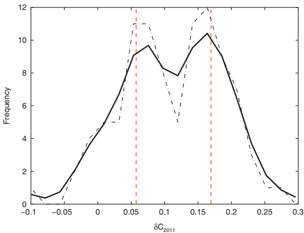
Figure 3 Frequency distribution, raw and smoothed, showing the CN bimodality in the 47 Tuc survey using the \delta C_{2011} values. The means of each population are shown as red lines.
