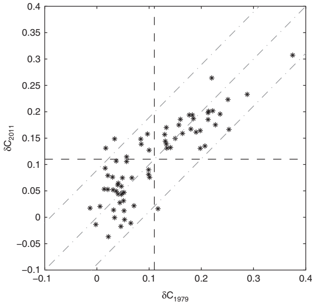
Figure 2 Comparison of CN excesses ( \delta C ), from NF79 and PF84 (on abscissa) with the values derived in this study (on ordinate). The dashed lines indicate the CN-weak/CN-strong threshold at \delta C = 0.11 . The dash-dot lines indicate the 1:1 relation \pm 2\sigma .
