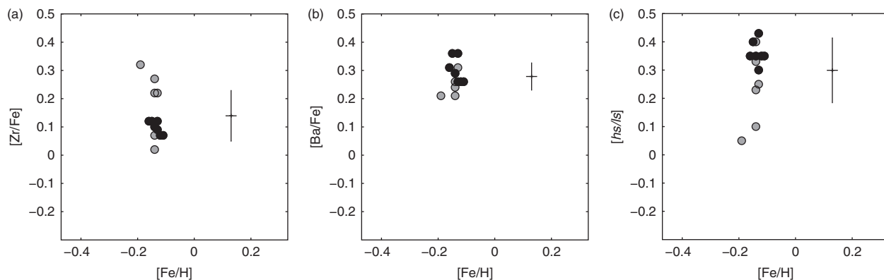
Figure 11 The abundances of the s -process elements with respect to Arcturus, (a) Zr and (b) Ba, against [\text{Fe}/\text{H}] for the thirteen Lee 2525-like stars in the 47 Tuc medium-resolution survey with sample mean and standard deviation. (c) The ratio of [\text{hs}/\text{ls}] against [\text{Fe}/\text{H}] for the sample. Grey circles are CN-weak stars and black circles are CN-strong.
