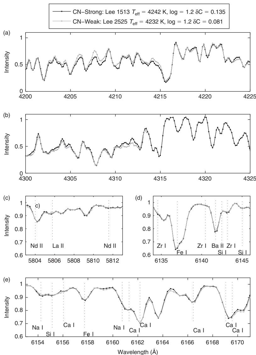
Figure 7 Comparison of Lee 2525 (grey) and Lee 1513 (black) spectra. (a) CN band, (b) CH band, (c) Nd II and La II, (d) Si I, Fe I, Ba II and Zr I, (e) Na I, Si I, Ca I and Fe I.
