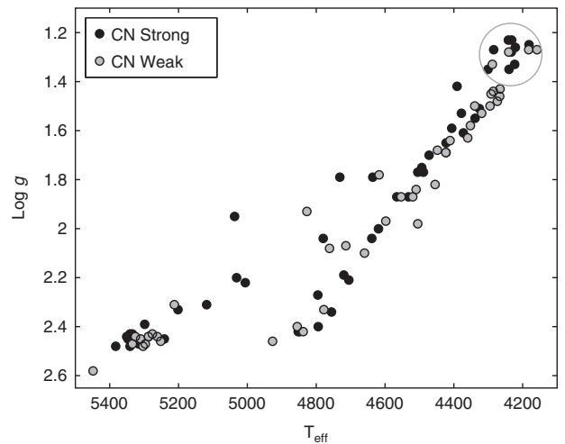
Figure 5 T_{\text{eff}} – \log g space for CN-weak (grey circle) and CN-strong (black circle) pairs based on V-K photometry. The circle encompasses Lee 2525-like stars.
