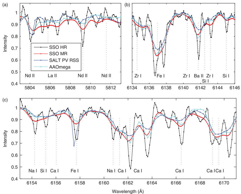
Figure 6 Comparison of the Lee 2525 spectra observed using RSS on SALT (blue), the SSO 2.3-m telescope (black), and AAOmega on the AAT (cyan). Also included is the convolution of the high-resolution spectra to a resolution comparable to the AAOmega observation (red). (a) Nd II and La II features in the 5800 Å region. (b) Si I, Fe I, Ba II and Zr I features in the 6140 Å region. (c) Na I, Si I, Ca I and Fe I features in the 6160 Å region.
