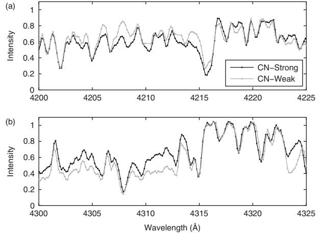
Figure 4 Comparison of a CN-weak star (grey, Lee 4506, \delta C_{2011} = 0.050 ) with a CN-strong star (black, Pal 578, \delta C_{2011} = 0.164 ) of similar T_{\text{eff}} and \log g from the 47 Tuc stellar survey. (a) CN bandhead at 4216 Å. (b) G Band.
