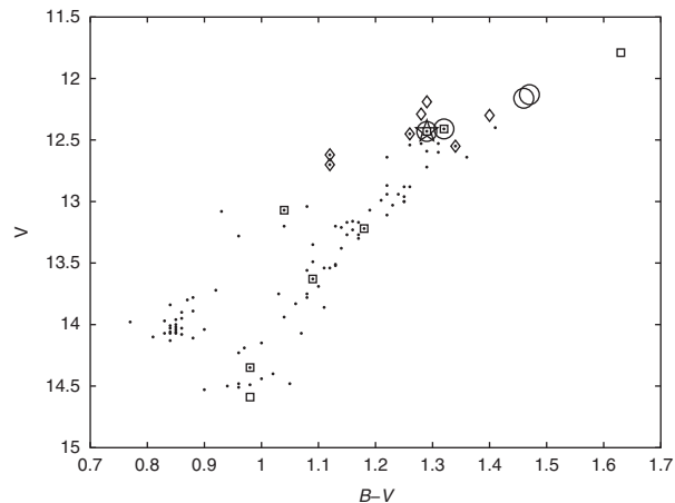
Figure 1 Colour-magnitude diagram of the 47 Tuc stars observed in the AAOmega medium-resolution survey (●). Stars from Brown & Wallerstein (1992) (○), Wylie et al. (2006) (◇) and Worley et al. (2008) (□), as well as Lee 2525 (star) are shown.
