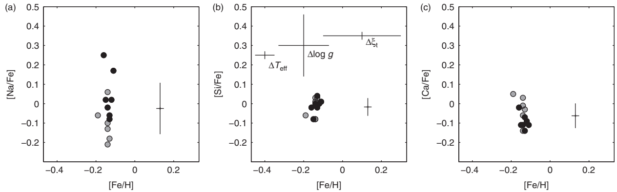
Figure 9 The element abundance ratios [X/Fe] calculated with respect to the medium-resolution abundance analysis of Arcturus for (a) Na, (b) Si and (c) Ca, against [Fe/H] for each of the 13 ‘Lee 2525-like’ stars. Grey circles are CN-weak stars and black circles are CN-strong. The sample mean and standard deviation for each is also shown. The systematic uncertainties from Table 4 are illustrated for [Si/Fe] .
