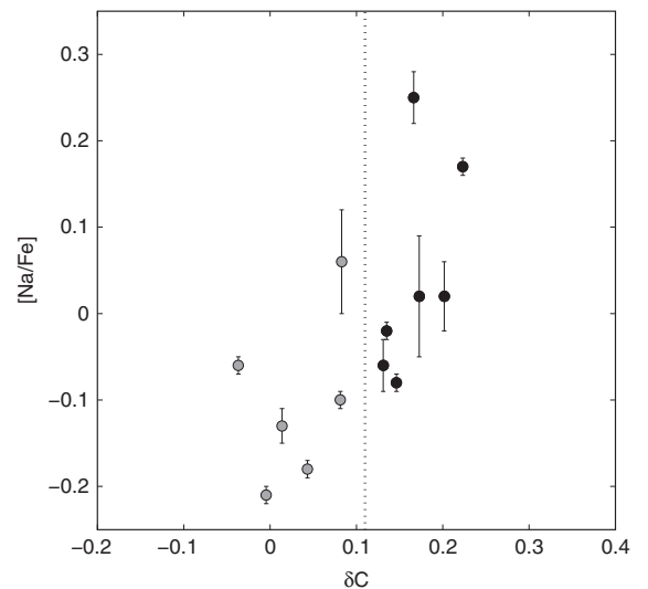
Figure 10 [Na/Fe] with respect to Arcturus against \delta C_{2011} for each of the thirteen Lee 2525-like stars. The dotted line shows the threshold at 0.11. Grey circles are CN-weak stars and black circles are CN-strong.
