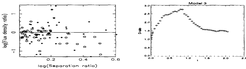
Figure 2. (a) observed r_D (Separation ratio)- r_L (Flux density ratio) diagram filled - quasars, unfilled - galaxies; (b) simulated r_D with time.
