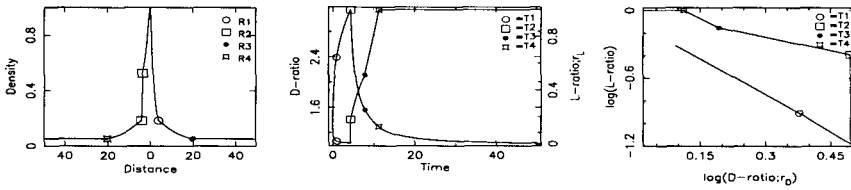
Figure 1. Analytical model: density (a), r_D and r_L (b), r_D - r_L (c).
