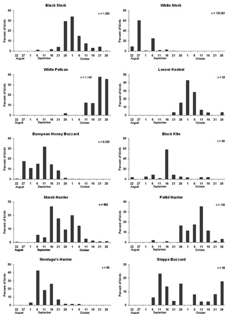
Figure 2. Timing of soaring and gliding migrants at Zeit Bay between 20 August and 28 October 2006. The graphs are based on the daily number of birds per observation hour.
