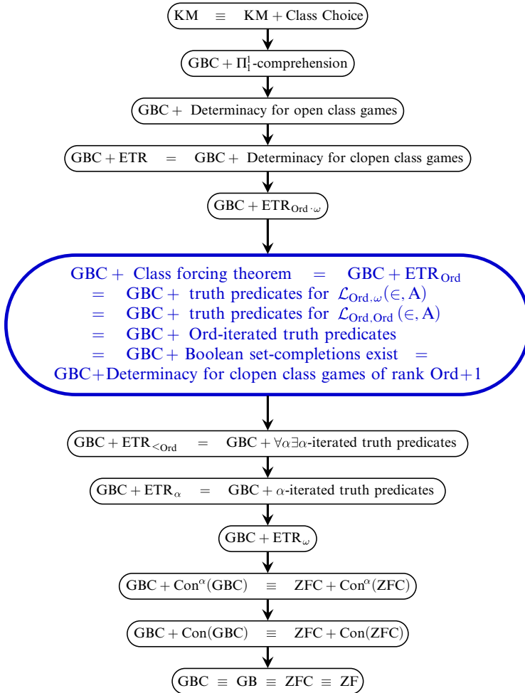
FIGURE 1. A hierarchy of theories between GBC and KM by consistency strength ( \equiv means equiconsistent)
