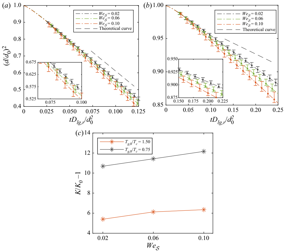
Figure 12. Time history of (d/d_0)^2 when varying the Weber number, We_S = 0.02 - 0.06 - 0.10 and for temperature ratios (a) T_{g,0}/T_c = 1.50 and (b) T_{g,0}/T_c = 0.75 . The black dashed curves represent the theoretical prediction of the actual evaporation rate obtained with the procedure explained in § 4.1. The length of the error bars (included for tD_{lg,r}/d_0^2 > 0.025 and tD_{lg,r}/d_0^2 > 0.04 , respectively) indicates the droplet with the fastest/slowest evaporation rate among the five droplets in the simulations. (c) Evaporation enhancement (i.e. K/K_0 ) as a function of We_S for Re_S = 6700 and T_{g,0}/T_c = 0.75 - 1.50 .
