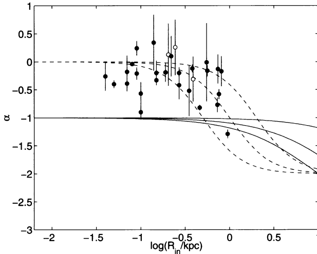
Figure 1. The power-law slopes, \alpha , of the central mass-density profiles, \rho \propto r^\alpha derived from the five innermost data points of the rotation curves of our three target objects (open symbols). Filled symbols indicate the de Blok & Bosma (2002) measurements. R_{\text{in}} represents the radius of the innermost data point used in the fit. The three dashed lines indicate the slopes predicted by pseudo-isothermal spheres with core radii of 0.5, 1 and 2 kpc, whereas the solid lines represent the Navarro et al. (1996) CDM predictions for characteristic halo radii of 10, 20 and 100 kpc.
