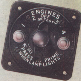
C.1820-Y Type PRIMING SWITCH for 2 or 4-engined Aircraft
