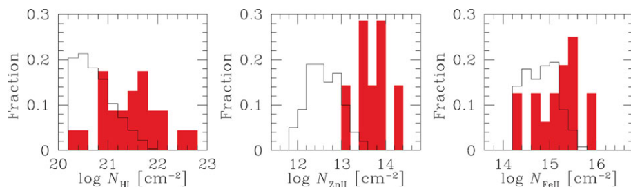
Figure 2. Fraction of QSO-DLAs (empty histograms) or GRB-DLAs (filled histograms) per column density bins for different ions (from left to right: HI, ZnII and FeII).
