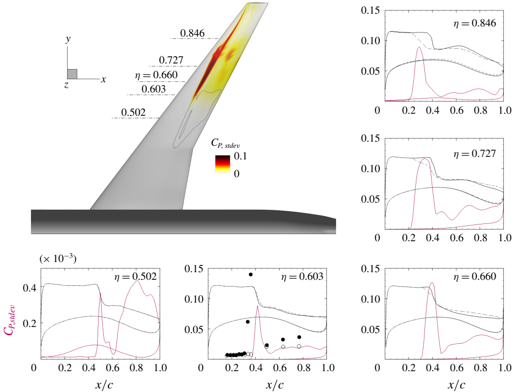
FIGURE 17. Standard deviation of surface pressure coefficient, C_{p,stdev} , in the nonlinear regime, computed in a duration of approximately 30 non-dimensional time units, over the entire wing surface and selected outboard spanwise stations. Pressure coefficients of base flow (solid black line) and mean flow (dashed dark grey line) are included for orientation. Also shown is mean-flow reverse-flow region in the surface plot (dark grey line). Experimental root-mean square data of pressure fluctuations for spanwise station \eta = 0.603 at angles of attack \alpha = 3.35^\circ ( \circ ) and 3.88^\circ ( \bullet ) were taken from Koike et al. (2016) (at Re \approx 1.5 \times 10^6 ) to bracket \alpha = 3.75^\circ discussed herein.
