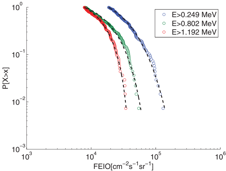
Figure 1. Extreme value analysis for three energy channels. Cumulative distribution from observations (circles) and associated fitted GP functions (dashed)
