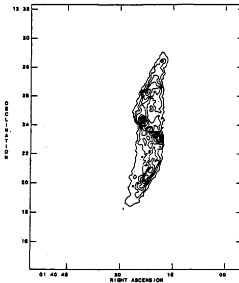
Figure 4: The integrated HI flux of NGC 660. The peak flux observed is 1.6167 X 10 3 Jy/Beam*m/s and the contour levels are at 1.8615 X 10 2 X (1, 2, 3, 4, 5, 6, 7, 8) Jy/Beam*m/s. Owing to absorption at the center of the galaxy, there is a hole in the map.
