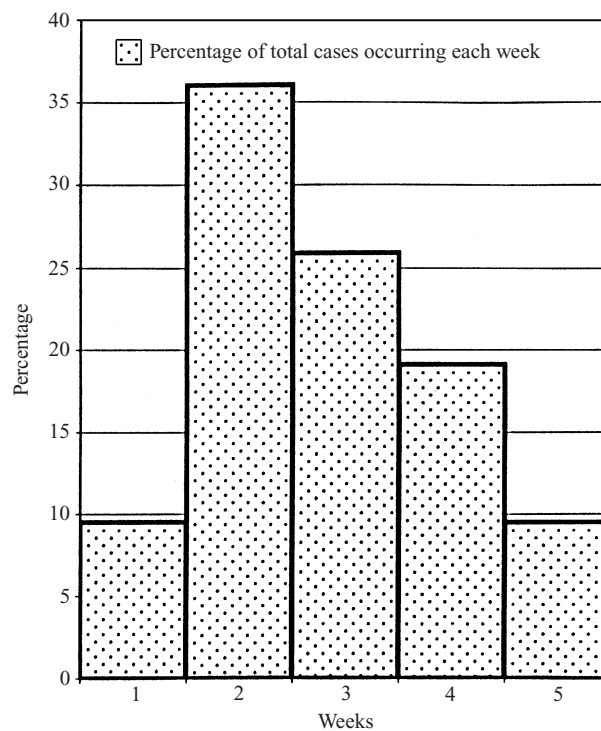
Fig. 2. Epidemic curve for village Ka, 1 July-8 August, 1991.
