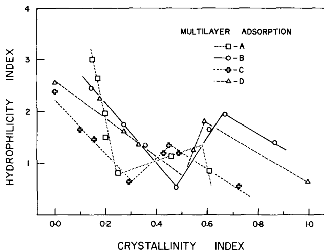
Fig. 3. Variation of multilayer hydrophilicity with crystallinity (Index, I_{021}/I_{060} ) and particle size.
