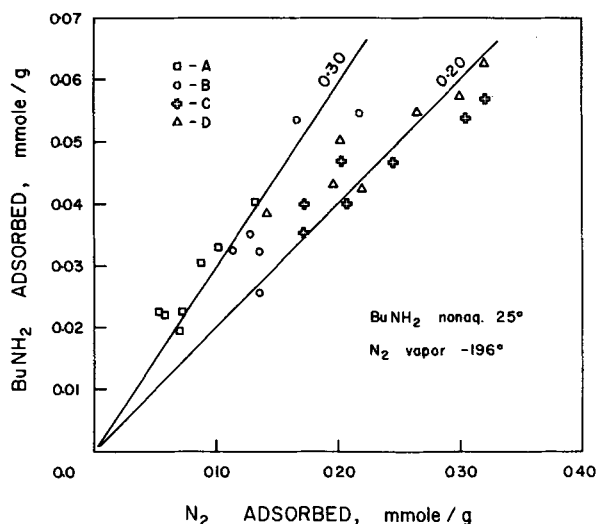
Fig. 5. Linear relationships between butylamine and nitrogen adsorption for monolayer coverage.
