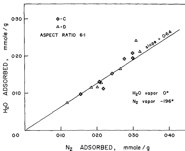
Fig. 4. Linear relationship between nitrogen and water vapor adsorption for monolayer coverage.
