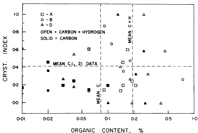
Fig. 1. Association of organic contamination with crystallinity (Index, I_{021}/I_{060} ).
