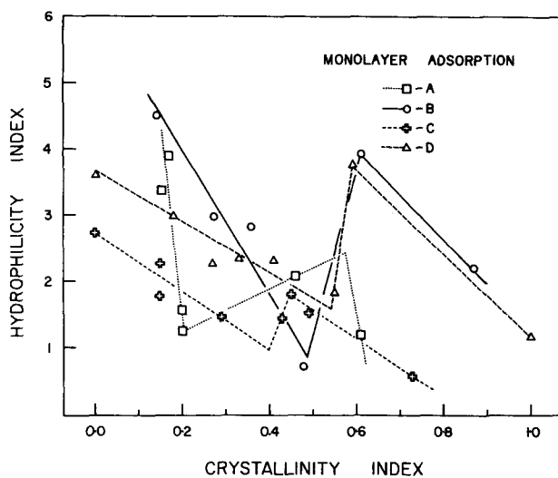
Fig. 2. Variation of monolayer hydrophilicity with crystallinity (Index, I_{021}/I_{060} ) and particle size.
