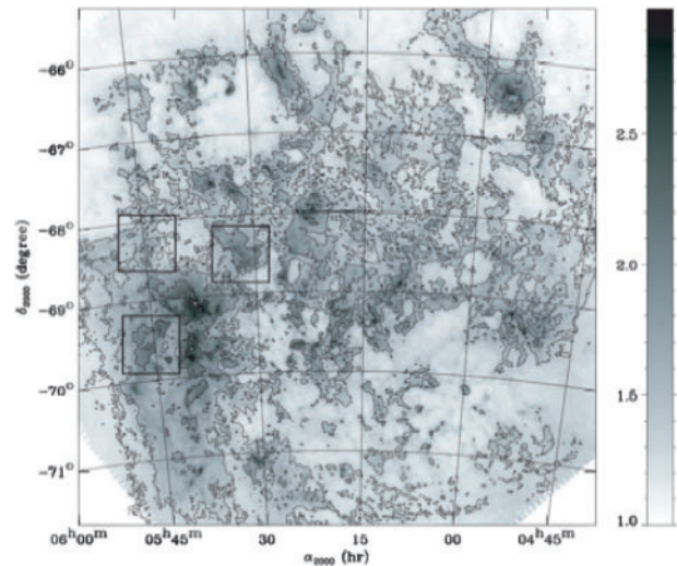
Figure 6 The distribution of H \alpha gas, shown in contours (Kim et al. 2003), compared with MIPS 160- \mu m emission (greyscale) of the LMC with (from Bernard et al. 2008). The square boxes outline regions analyzed in more detail by Bernard et al. (2008) to derive dust-to-gas mass ratios.
