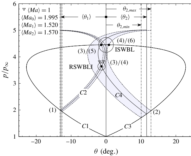
FIGURE 24. (Colour online) Shock polar for \theta = 13^\circ exhibiting separation shock variance from Matheis & Hicckel (2015) (notation altered for consistency).
