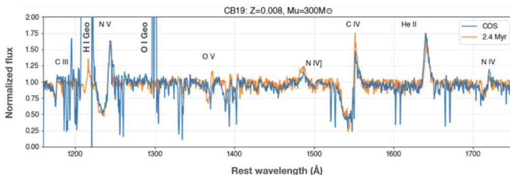
Figure 2. Comparison of COS G130M + COS G130M observation (blue curve) with best-fit model with VMS (orange curve). The strong emission lines at around 1210 and 1300 Å are due to Lyman-alpha and O I geocoronal emission.
