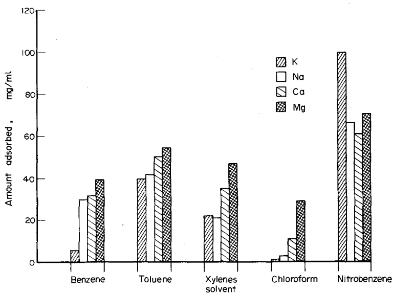
Figure 6. Adsorption of SDAB onto montmorillonite as a function of solvent and exchangeable cation at 0.5 mg/ml initial concentration.
