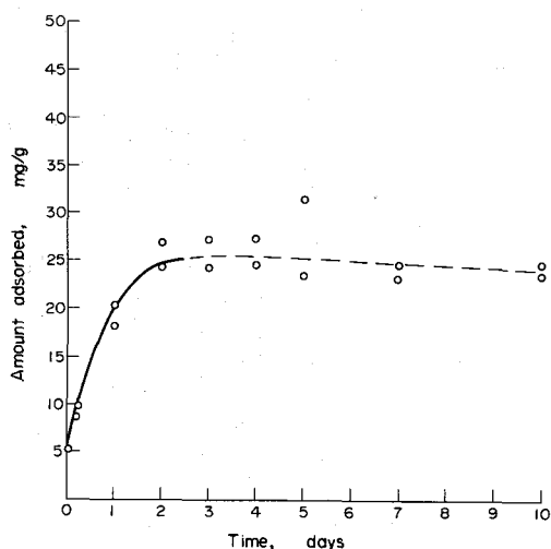
Figure 2. Adsorption of SDA bottoms onto \text{Na}^+ -montmorillonite in benzene as a function of time at 1 mg/ml initial concentration.
