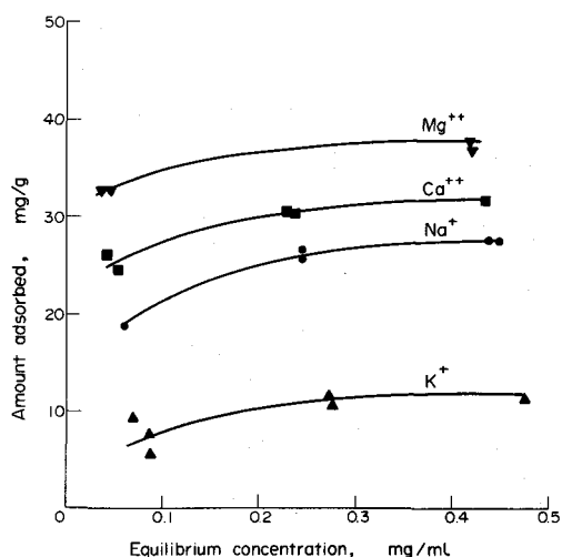
Figure 5. Adsorption of SDAB onto montmorillonite from benzene solution as a function of exchangeable cation.
