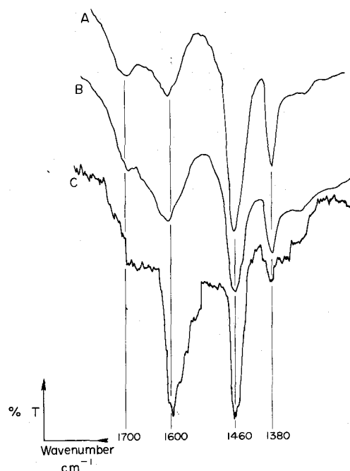
Figure 4. I.r. spectra of: A—pentane soluble SDAB fraction, B—pentane insoluble SDAB fraction, C—adsorbed SDAB on \text{Na}^+ -montmorillonite.
