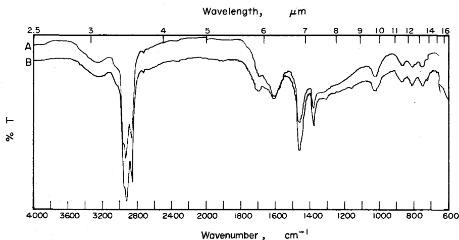
Figure 1. I.r. spectra of pentane insoluble (A) and pentane soluble (B) fractions of SDAB.
