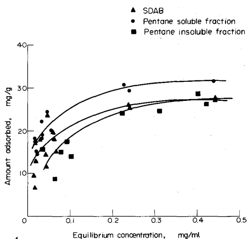
Figure 3. Adsorption of SDAB and component fractions onto \text{Na}^+ -montmorillonite from benzene solution.
