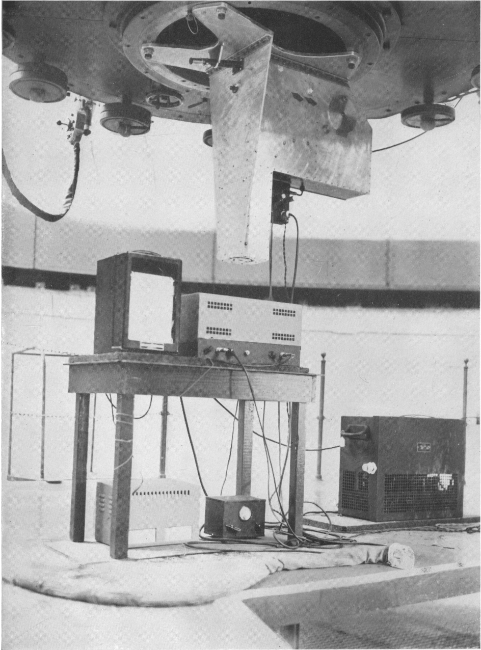
Fig. 1. Infra-red equipment at McDonald Observatory. Top: 82 in. cell + spectrometer and pre-amplifier. On table: amplifier (right) and recording meter. On floor (right): constant frequency unit with oscillating crystal; 60 cycles per sec. output, accurate to 1: 200,000. Under table: control box of above unit, and (left) condenser box, to lengthen period of recording meter at will from \frac{1}{2} -6 sec.
