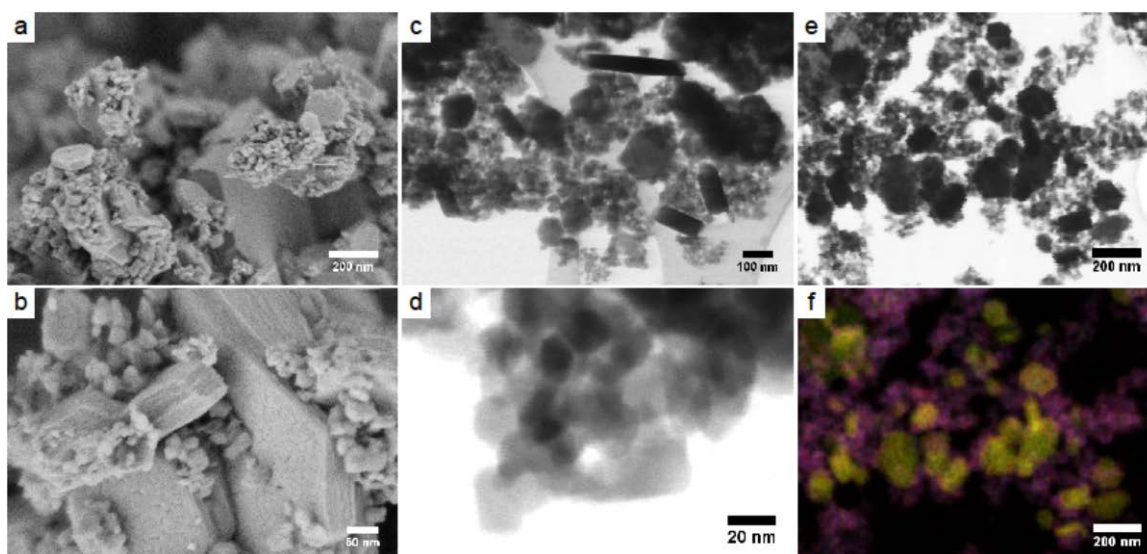
Figure 2. (a, b) Secondary electron micrographs with landing voltage of 1 kV in deceleration mode with the upper detector, (c, d) bright-field STEM micrographs at E_0 = 30 kV and (e, f) bright-field STEM micrograph and its corresponding EDS-x-ray map showing the \text{Li}_2\text{CoSiO}_4 nanoparticles in pink and the CoO by-product particles in yellow. All micrographs were from a \text{Li}_2\text{CoSiO}_4 nanopowder used as a cathode material for LIB.
