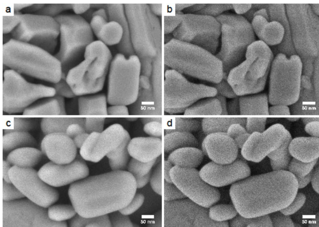
Figure 1. Secondary electron micrographs of a pristine LPF powder (a, b) and the same LPF powder with a surface carbon layer (c, d) recorded at E_0 = 2 kV with a stage bias of 10 V (landing energy of 1.9 kV). (a, c) Upper in-lens detector, (b, d) top in-lens detector without energy filtration.
