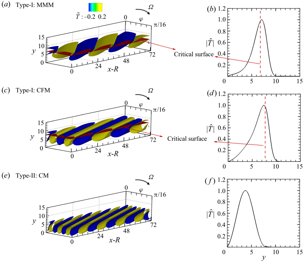
Figure 18. (a,c,e) Iso-surfaces of \tilde{T} and the (b,d,f) |\hat{T}| -profiles for the most unstable modes of the three types of instabilities for \tilde{\Omega} = 0.75 and X = 1 . (a,b) MMM with \alpha = 0.17 - 0.009i , \beta = 0.1 and \omega = 0.08 ; (c,d) CFM with \alpha = 0.18 - 0.0059i , \beta = 0.23 and \omega = 0 ; (e,f) CM with \alpha = 0.37 - 0.0062i , \beta = 0.4 and \omega = 0 . The critical surfaces in panels (a–d) denote the positions where \tilde{U} = c_r .
