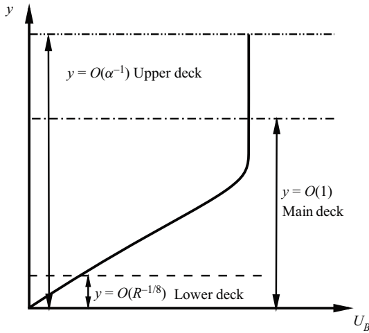
Figure 28. Asymptotic structure of the viscous-inviscid-interactive (triple-deck) instability.
