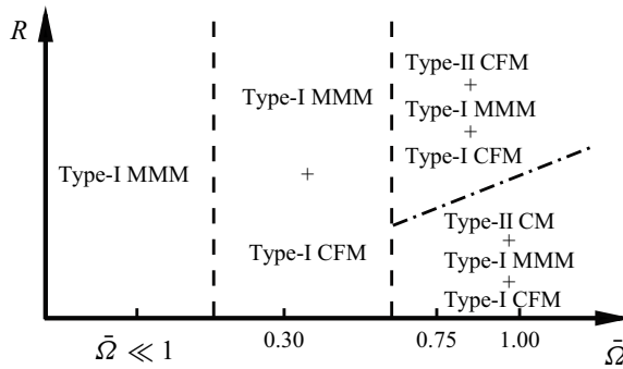
Figure 26. Different instability mechanisms in the R – \bar{\Omega} plane.
