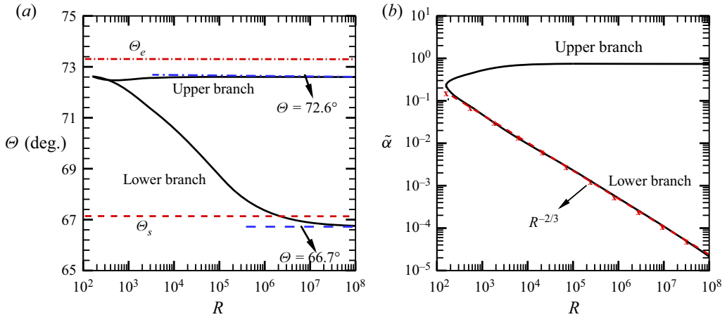
Figure 12. The neutral curves of the stationary CFM in the (a) \Theta - R plane and the (b) \tilde{\alpha} - R plane. The red dot-dashed line and dashed line in panel (a) represent \Theta_e = 73.3^\circ and \Theta_s = 67.1^\circ , respectively. The red dashed line with crosses in panel (b) denotes the power law R^{-2/3} .
