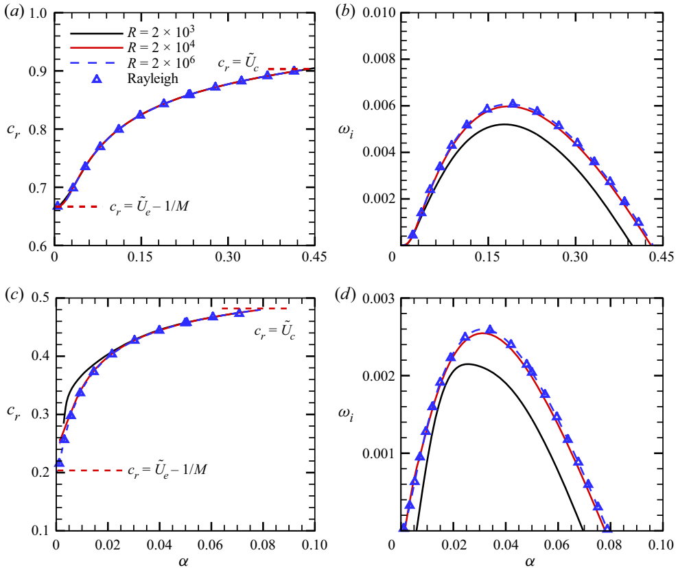
Figure 10. Dependence on \alpha of the phase speed c_r and the temporal growth rate \omega_i for MMM. The first and second rows denote the results for \Theta = 0^\circ and -75.9^\circ , respectively. Curves, O-S solutions; triangles, Rayleigh solutions.
