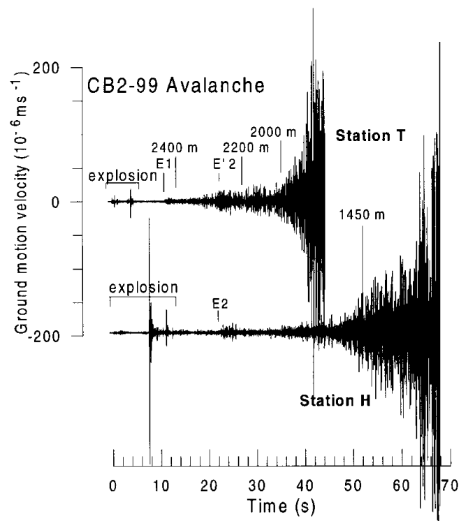
Fig. 7. First part of the seismograms of the 1999 Crêta Besse (CB2-99) avalanche recorded at stations T ( N-S component) and H ( W-E component). E1, E2 and E'2 correspond to earliest avalanche signals detected. The arrival times at different heights are indicated according to the arrival times deduced from Doppler radar and video measurements (personal communication from D. Issler, U. Gruber, N. Dawes and F. Dufour, 2000).
