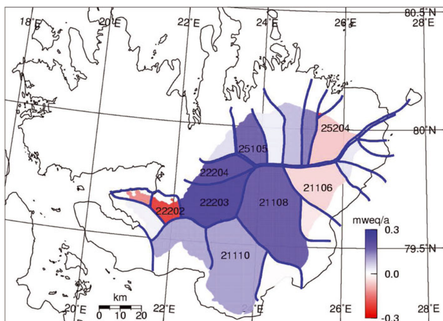
Fig. 2. Basin mean local mass balance. Shown in blue are those basins for which the mean local mass balance was positive, and in red those for which it was negative.
