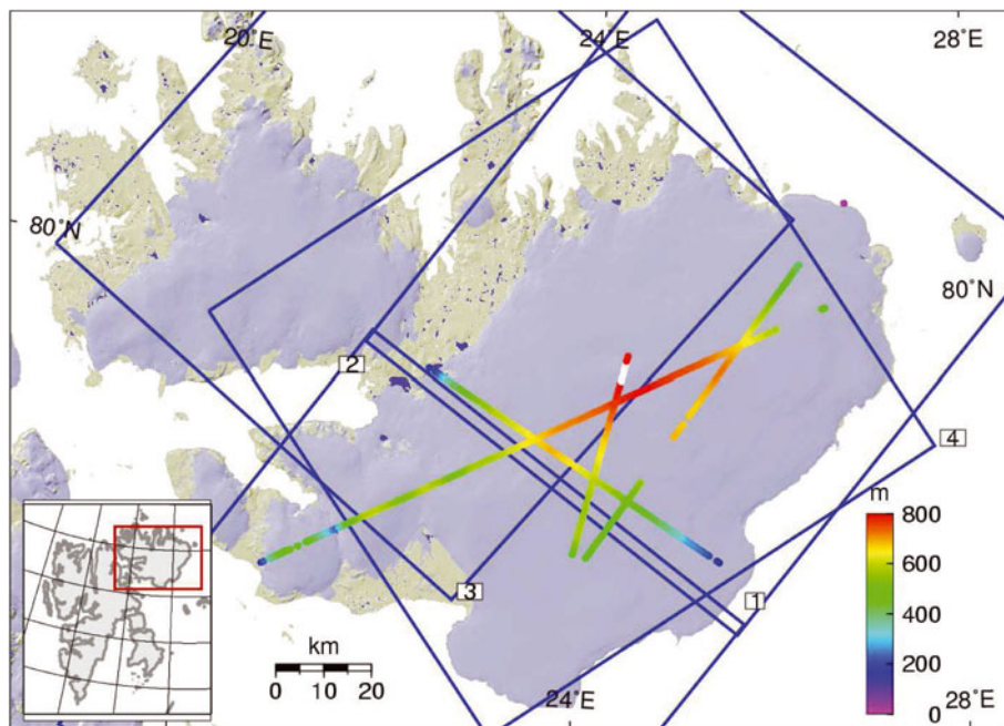
Fig. 1. Airborne laser altimeter data points (personal communication from J. Bamber, 2005), and location of data frames listed in Table 1. Inset shows location of Nordaustlandet within Svalbard.
