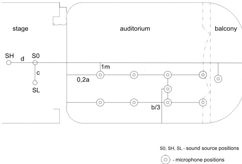
Figure 1. Microphone and sound source placement based on Takenaka R&D Institute methodology (Hidaka et al. 1995).
