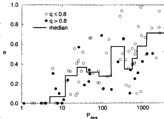
Fig. 5. The period–eccentricity diagram of the extended sample. The median eccentricity is indicated for bins containing 8 SB, starting from P = 5 days, and with 9 SB in the last bin.
