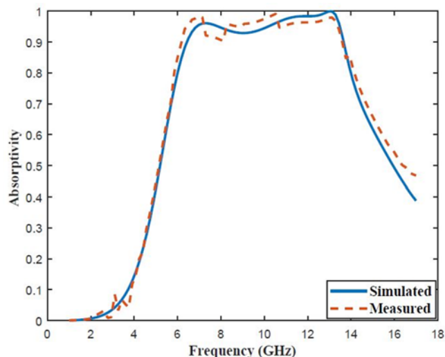
Figure 19. Simulated and measured absorptivity plot.
