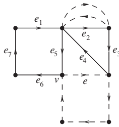
Figure 5.16 A nonmaximal tour in a balanced digraph
