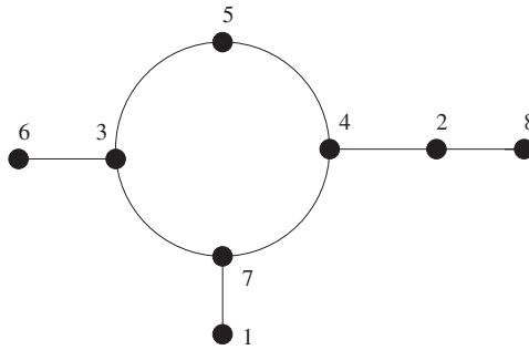
Figure 5.1 A circular arrangement of lines
