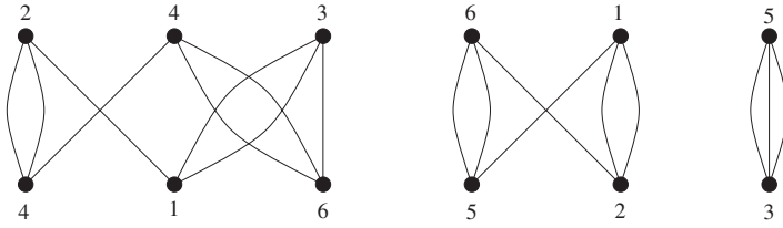
Figure 5.15 A bipartite graph \Gamma(A)
