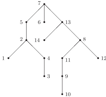
Figure 5.21 A recursively labelled tree
