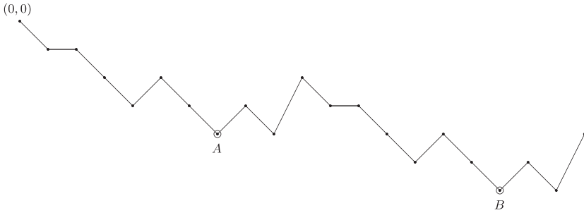
Figure 5.13 A lattice path LP(w^2)
