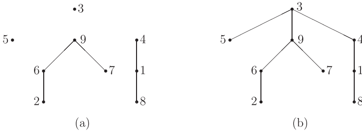
Figure 5.6 A plane tree built from the subtrees of its root
