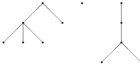
Figure 5.12 A plane forest of type (7, 2, 2, 1)
