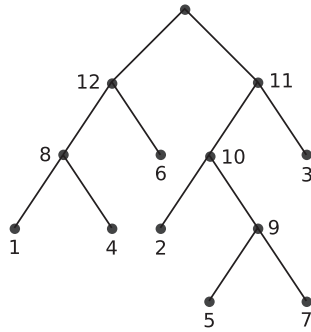
Figure 5.5 A decreasing labelled tree corresponding to a binary total partition
