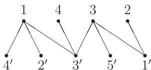
Figure 5.25 A labelled bipartite tree
