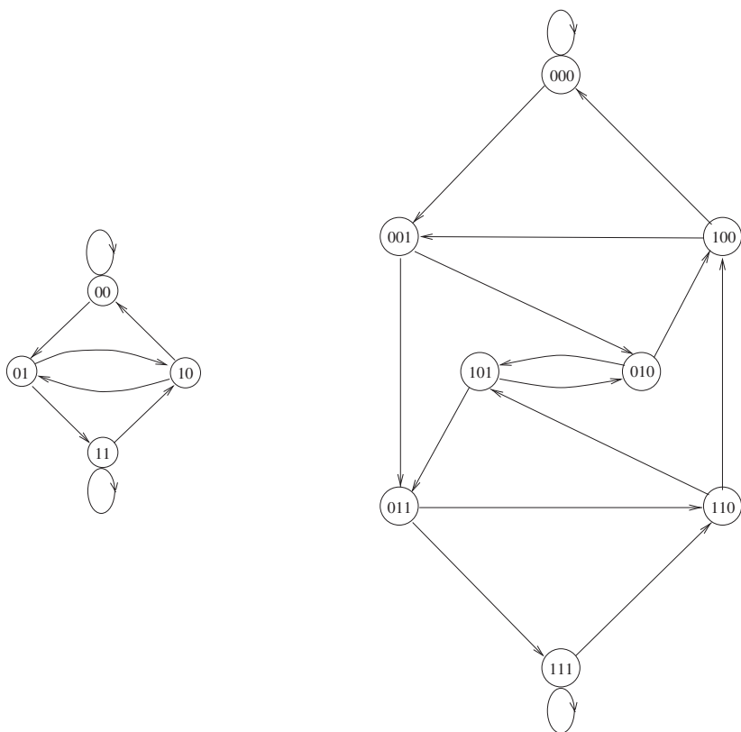
Figure 5.17 The de Bruijn graphs D_3 and D_4
