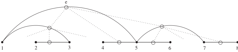
Figure 5.28 A ternary tree constructed from a noncrossing tree
