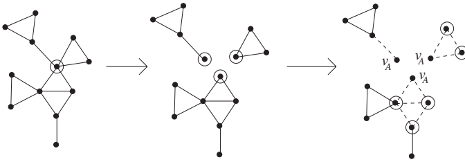
Figure 5.24 The block-tree decomposition
