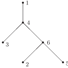
Figure 5.22 A tree with four inversions
