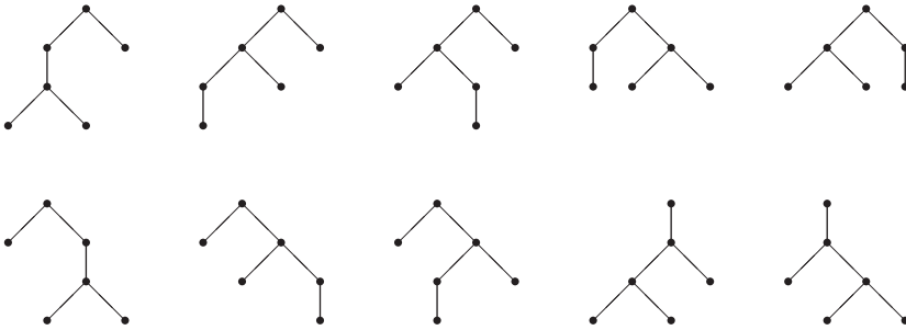
Figure 5.11 The ten plane trees of type (3, 1, 2)
