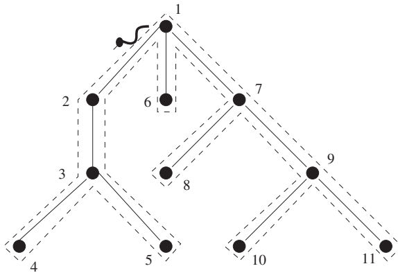
Figure 5.14 A plane tree traversed in preorder
