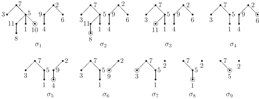
Figure 5.7 Constructing the Prüfer sequence of a labelled forest
