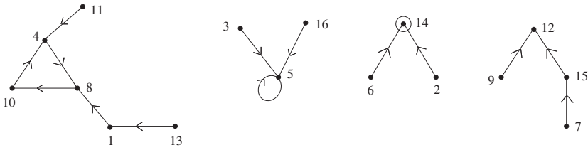
Figure 5.10 The digraph D(\sigma, i)
