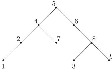
Figure 5.20 A local binary search tree.
