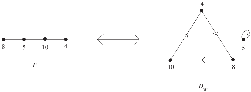
Figure 5.9 Two graphical representations of a permutation
