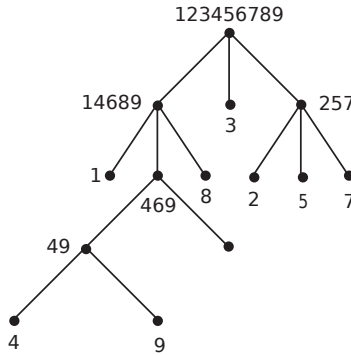
Figure 5.3 A total partition of [9] represented as a tree
