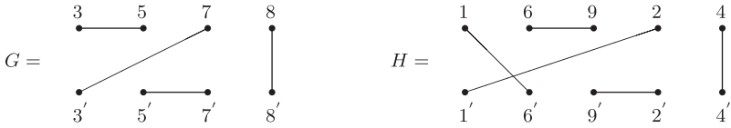
Figure 5.23 A pair of 1-factors
