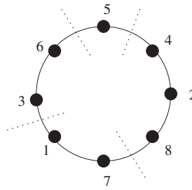
Figure 5.2 An equivalent form of Figure 5.1
