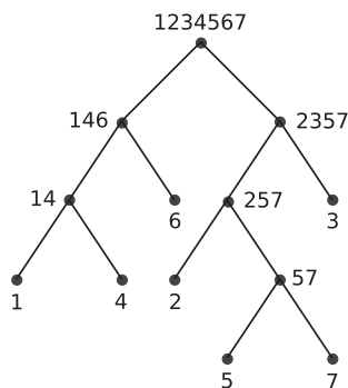
Figure 5.4 A binary total partition represented as a tree
