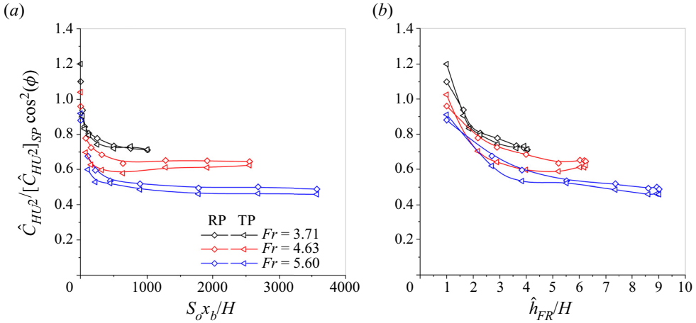
Figure 11. The relative wave force coefficient \hat{C}_{HU^2}/\{\hat{C}_{HU^2}\}_{SP}[\cos\phi]^2 for the RP and TP, corrected by the direction-cosine square. The dependence of the relative coefficient on (a) the position S_o x_b/H and undisturbed-flow Froude number Fr , and (b) the amplitude of the front runner \hat{h}_{FR}/H . The symbols \diamond and \triangleleft denote the data for RP and TP, respectively.
