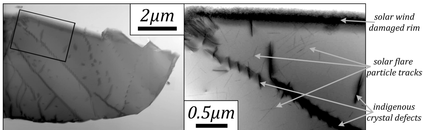
Figure 3. Bright-field images (BFIs) of section 1, after being lifted out and thinned to \sim 100\text{--}150\text{nm} . Features of space weathering (solar flare particle tracks, disordered rims, and nanophase particles decorating the outer edges) can be seen in the BFIs. (a) The entire section surrounded by epoxy; The C-cap is above the field of view, the TEM grid bar to the left. (b) Close-up of the area indicated in panel a.
