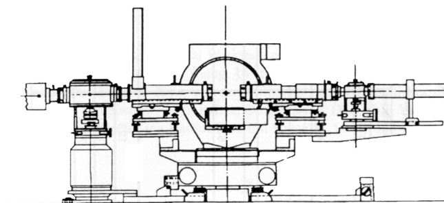
Huber 424/511.1 Sealed Source Beamline
