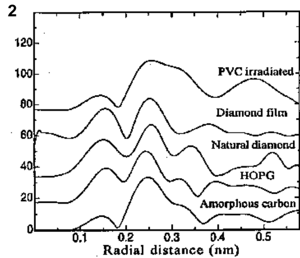
Figure 2. Radial Distribution Function corresponding to Fig. 1
