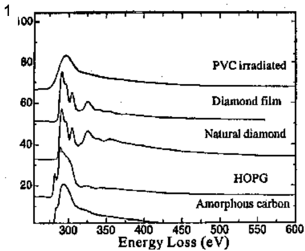
Figure 1. Extended fine structure in the transmission mode
