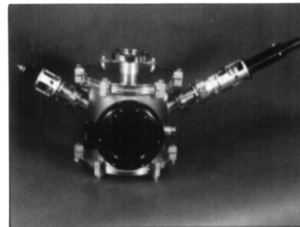
High-Speed In-Situ Ellipsometer
