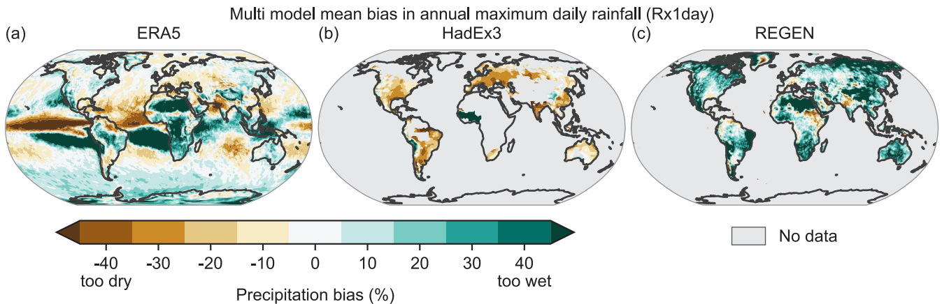
Figure 11.14 | Multi-model mean bias in annual maximum daily precipitation (Rx1day, %) for the period 1979–2014. Calculated as the difference between the Coupled Model Intercomparison Project Phase 6 (CMIP6) multi-model mean and the average of available observational or reanalysis products including (a) ERA5, (b) HadEX3, and (c) REGEN. Bias is expressed as the percent error relative to the long-term mean of the respective observational data products. Brown indicates that models are too dry, while green indicates that they are too wet. Areas without sufficient observational data are shown in grey. Adapted from Wehner et al. (2020) under the terms of the Creative Commons Attribution licence. Further details on data sources and processing are available in the chapter data table (Table 11.SM.9).
