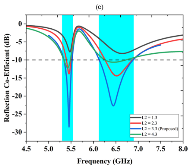
Figure 5. Parametric Study on parameters (a) L_4 , (b) L_5 , (c) L_2 .
