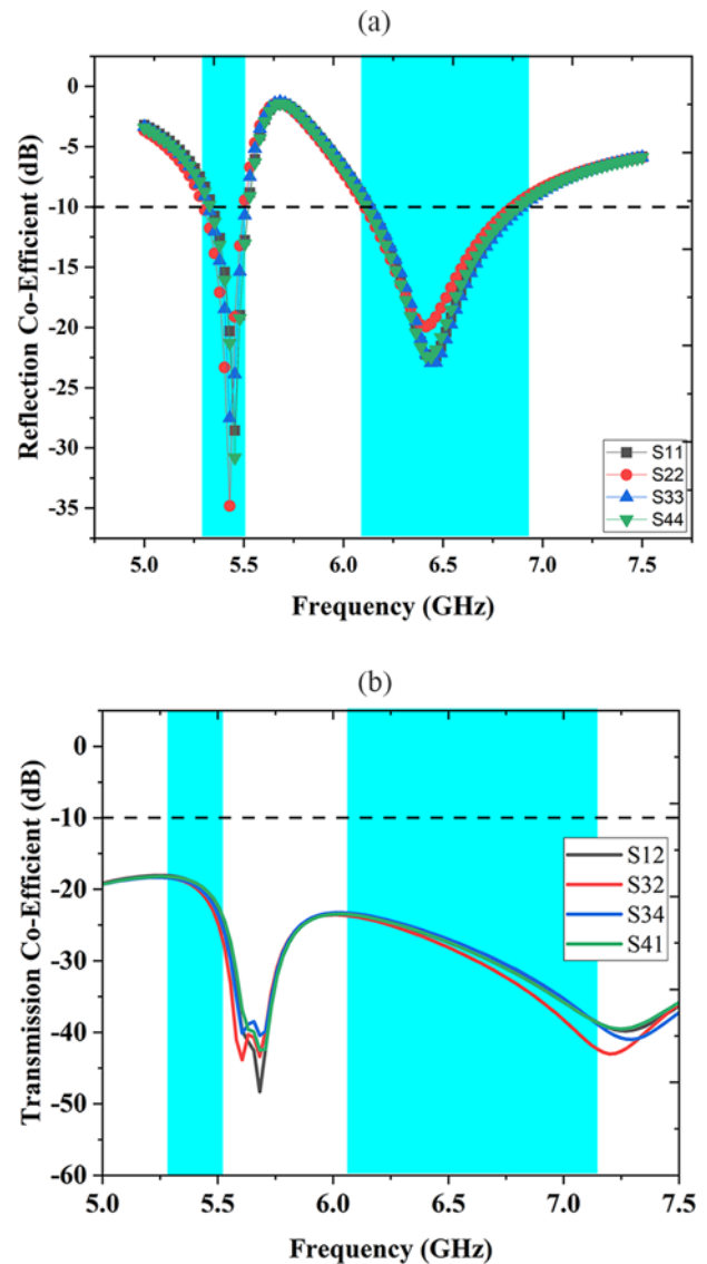
Figure 10. Measured (a) Reflection Co-Efficient, (b) Transmission Co-Efficient.
