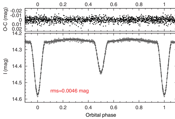
Figure 2. I -band light-curve solution to the SMC 108.1.14904 system. The rms of the residuals is at the level of the intrinsic photometric noise.
