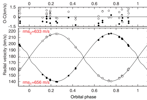
Figure 3. Radial-velocity solution to both components. The radial velocities of the primary (solid bullets) are blueshifted by -0.7 \text{ km s}^{-1} with respect to the secondary's velocities.
