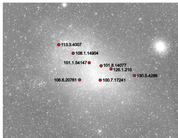
Figure 1. Eight late-type eclipsing binary stars in the SMC selected for distance measurements.
