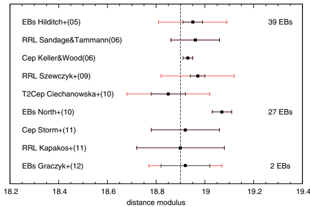
Figure 4. Recent distance measurements to the SMC. The ‘standard’ distance modulus to the SMC, (m - M)_0 = 18.90 mag, is also highlighted. The inner error bars denote statistical errors and outer error bars represent the systematic uncertainties. EBs: Eclipsing binaries.
