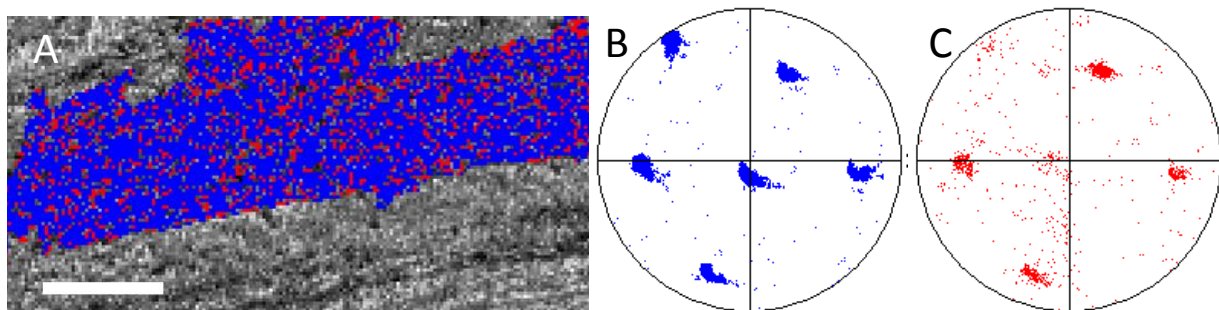
Figure 3. Example of EBSD results. A. Orientation map subset of one \beta -grain. Blue is for \beta -Ti and red is for \alpha -Ti. The plane of the image is perpendicular to the rolling direction. Scale bar is 10 \mu\text{m} . B. \{110\} pole figure of \beta -Ti. C. \{0001\} pole figure of \alpha -Ti. \{0001\}\alpha is parallel to \{110\}\beta . Two of 6 possible orientations of \alpha -Ti are not realized strongly.
