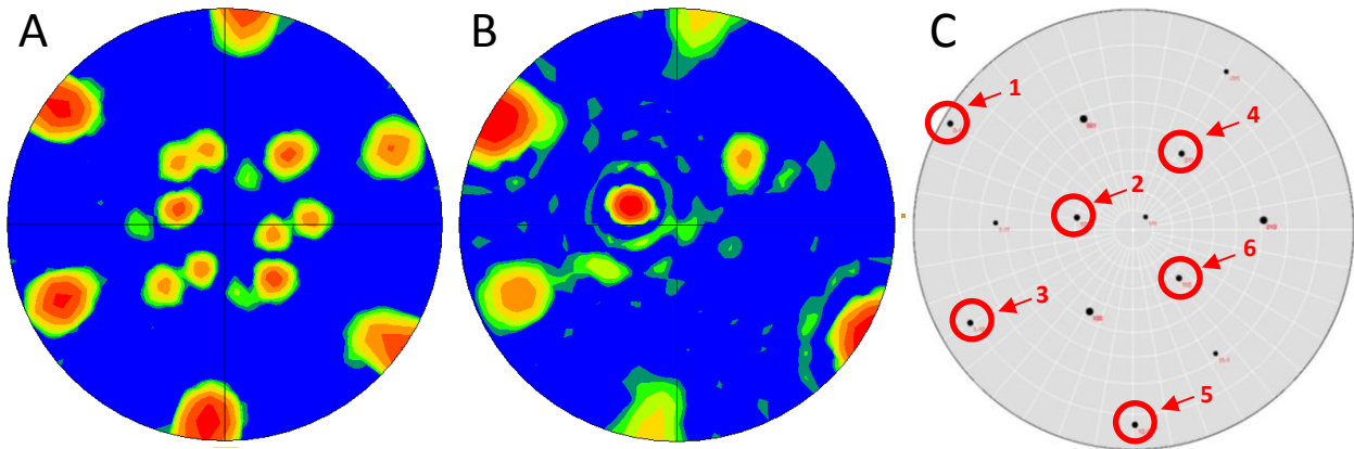
Figure 2. Pole figures obtained using PED of the area on the sample shown in Figure 1. A. \{110\} of \beta -Ti shows predominantly one orientation of \beta -phase parent grain. B. \{0002\} of \alpha -Ti shows that the vast majority of the \alpha -crystals have \{0001\}\alpha parallel to \{110\}\beta . C. Computer simulated pole figure of \{110\} of \beta -Ti shows that the realization probability of some OR variants within individual \beta -grains is not evenly distributed between all possible variants: variants 1 and 2 are the strongest, 3, 4 and 5 are medium and 6 practically not realized.
