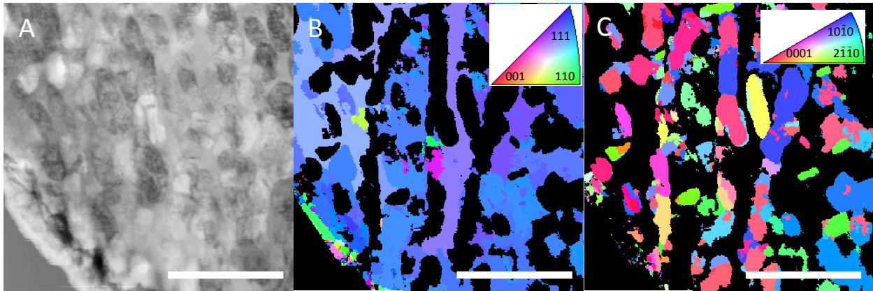
Figure 1. PED results on the crystal structure characterization of the phases involved during \beta \rightarrow \alpha transformation of VT22 alloy after severe hot plastic deformation. The e-beam is parallel to the rolling direction. Scale bar is 800 nm. A. Virtual bright-field image. B. Texture map for \beta -Ti shows essentially a single orientation for the \beta -phase parent grain, close to \{111\} . C. Texture map for \alpha -Ti shows a variety of grain orientations.
