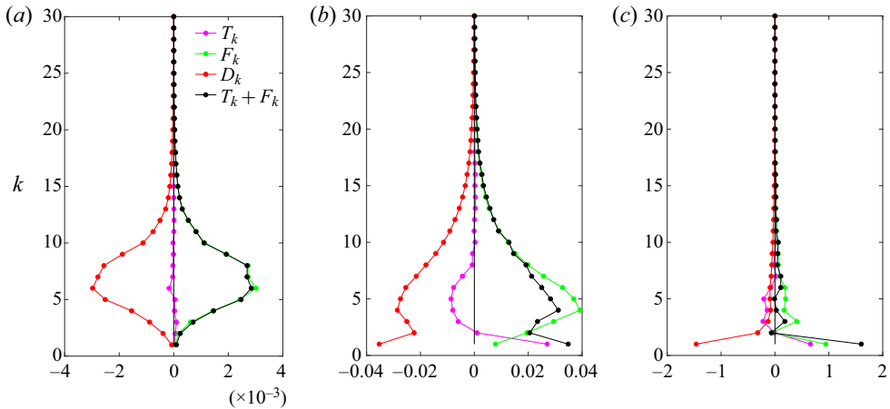
Figure 5. Time-averaged, barotropic transfer functions showing the change in energy transfer behaviour as the inverse cascade becomes more prominent. All cases use \tilde{Ra} = 60 and Prandtl numbers (a) Pr = 7 ( \tilde{Re} \approx 2.5 ), (b) Pr = 2.5 ( \tilde{Re} \approx 6.8 ) and (c) Pr = 1 ( \tilde{Re} \approx 16.8 ). These three cases are representative of, respectively, the CTC/ P regime, showing no LSVs in the domain and \tilde{Re} \ll 6 ; the P regime, showing LSVs in the domain and \tilde{Re} \gtrsim 6 ; the G regime, with robust LSVs and \tilde{Re} \gg 6 .
