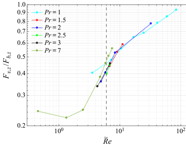
Figure 13. Ratio of the vertical components of the r.m.s. viscous force, F_{v,z} = \nabla_{\perp}^2 w , to the r.m.s. buoyancy force, F_{b,z} = \tilde{Ra} Pr^{-1} \vartheta , as a function of \tilde{Re} .
