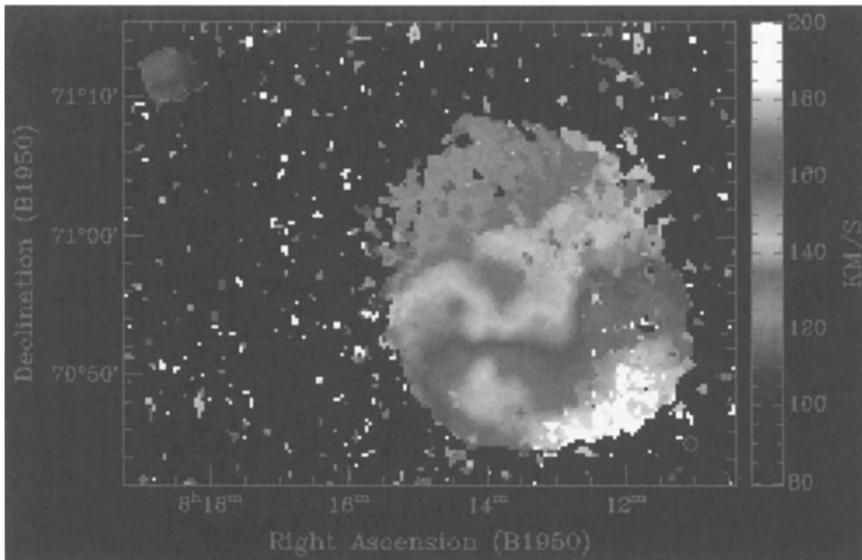
Figure 3. Intensity-weighted mean HI velocity field of the survey area near HoII and M81dwA.
