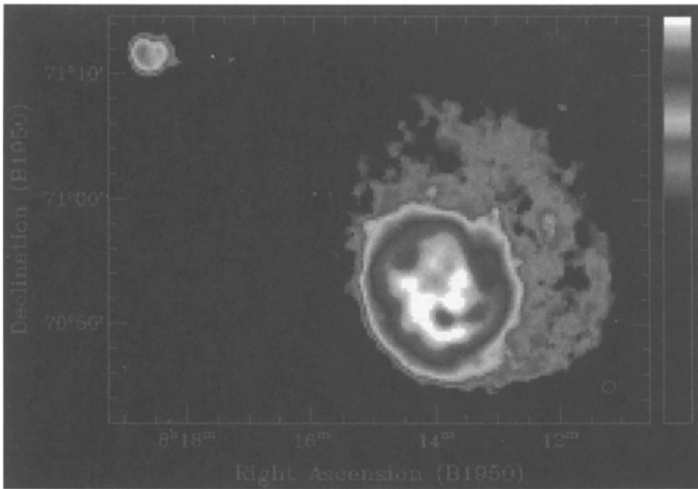
Figure 2. Total HI map of the survey area near HoII and M81dwA (logarithmic fluxes).
